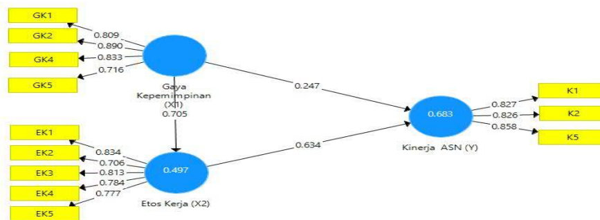
Gambar 1. Model PLS Algoritma
